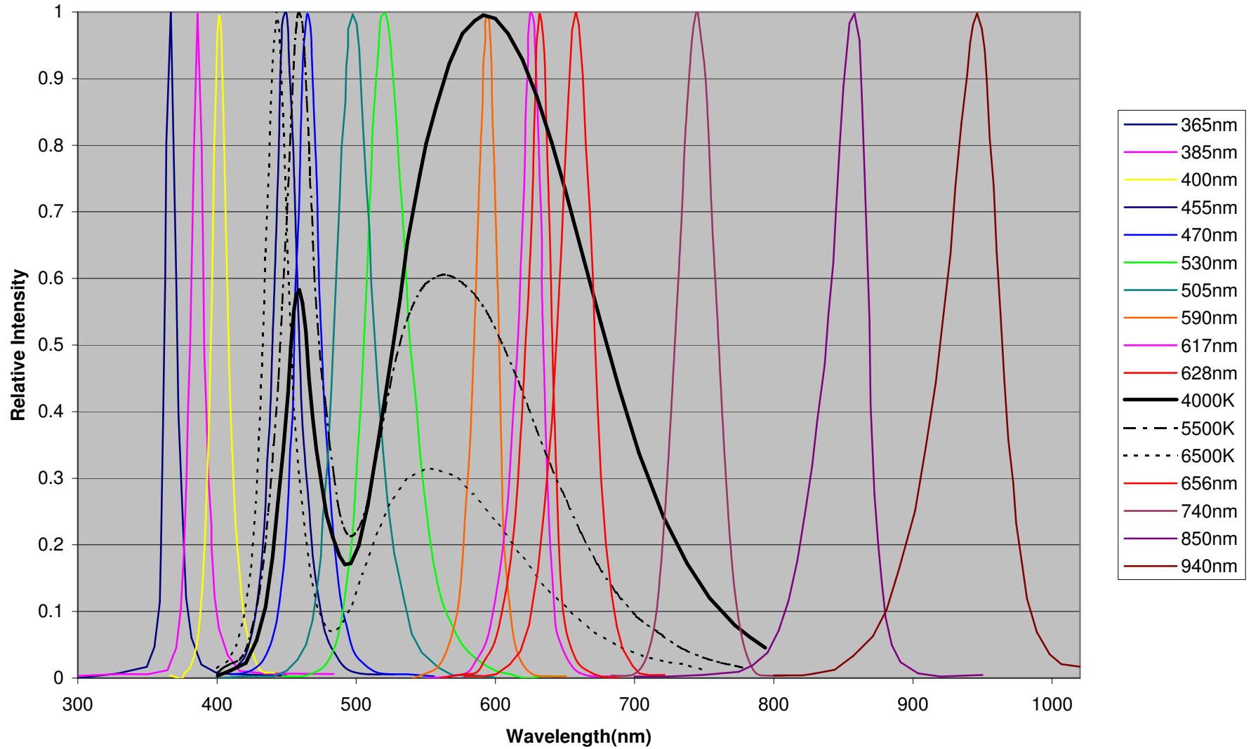
Mightex LED Typical Spectra
